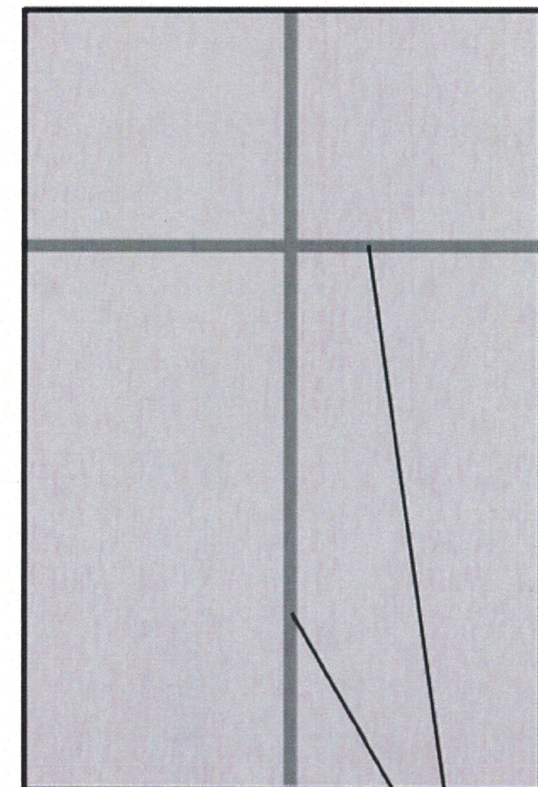
Discrete Fracture Representation
