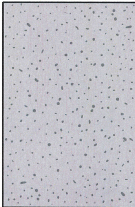
Equivalent Porous Medium Representation
