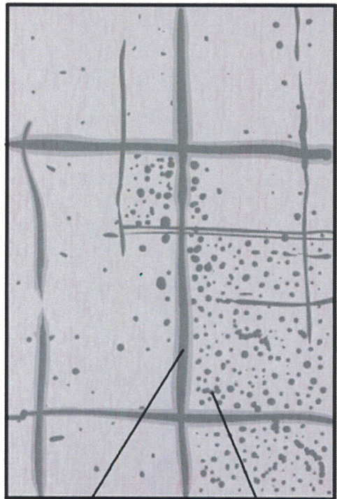
Fractured Bedrock
